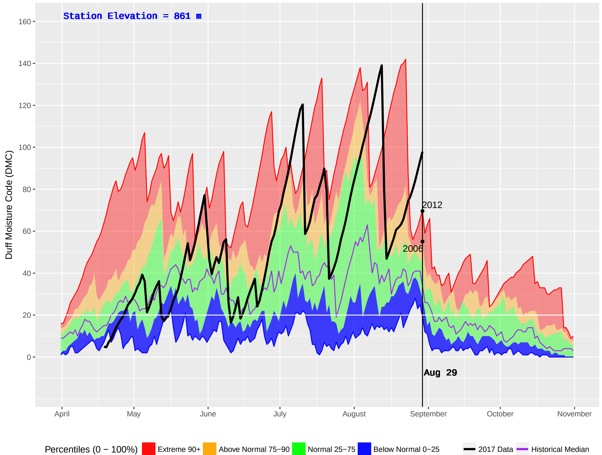
BLAEBERRY (866) : Historical (2004–2016) and Current (2017) Noon Duff Moisture Code (DMC)
