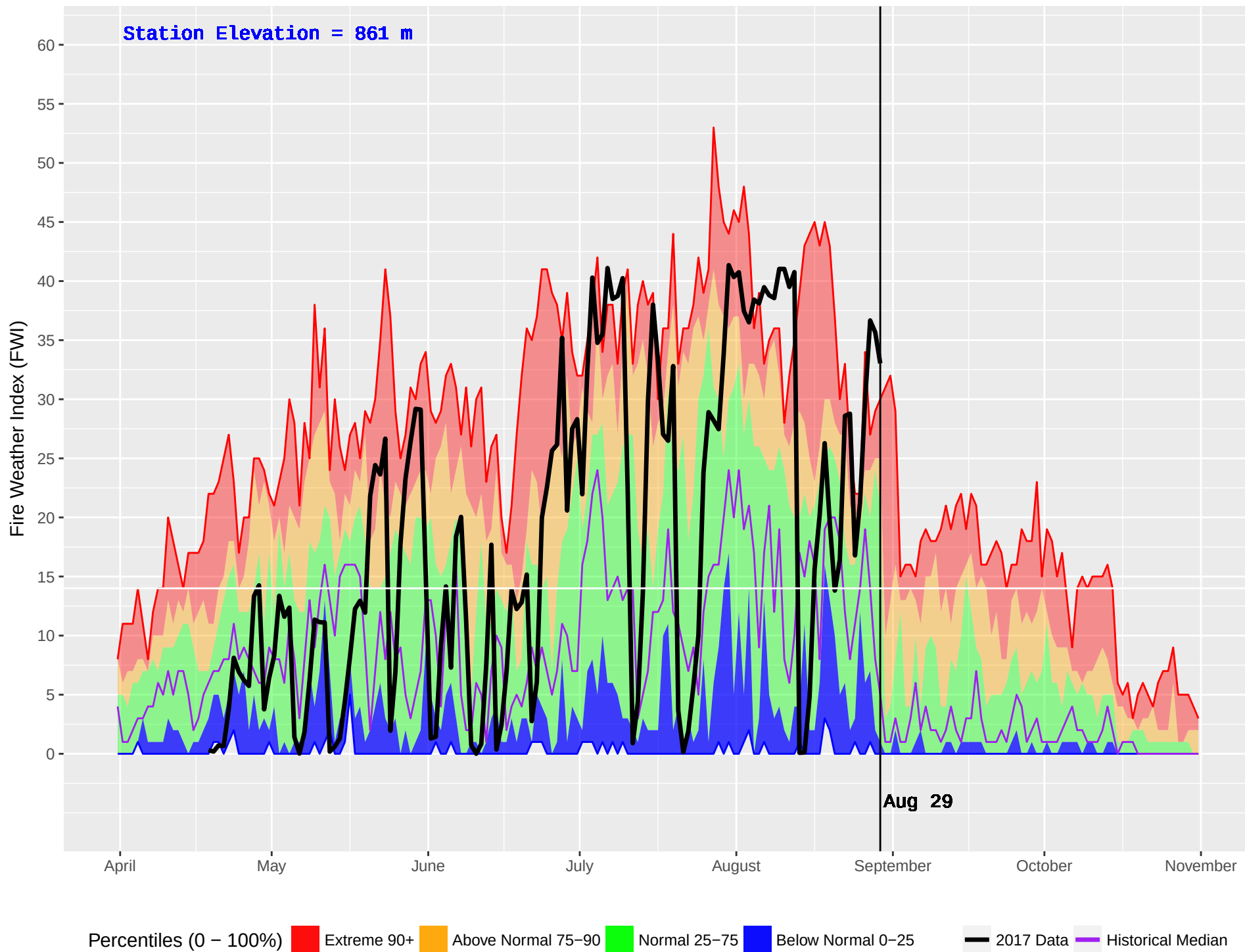
BLAEBERRY (866) : Historical (2004–2016) and Current (2017) Noon Fire Weather Index (FWI)
